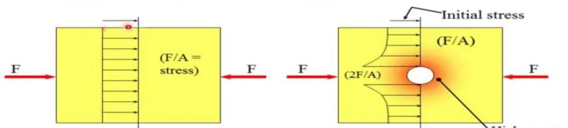
Figure 5. tangeres Plotting stresses around a borehole
