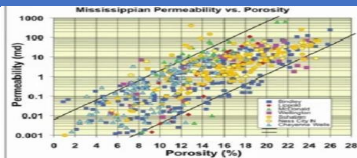
Figure 9. Porosity & permeability
